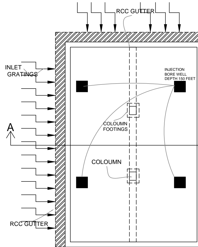
TOP SLAB PLAN
