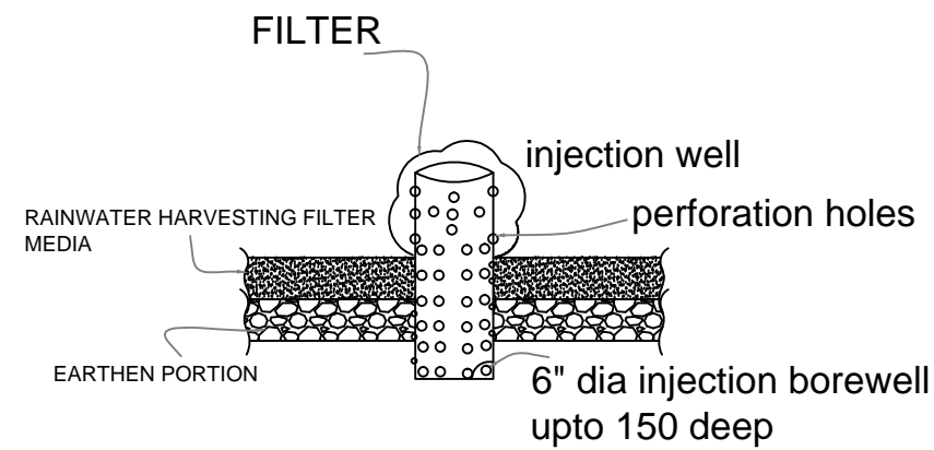
TYPICAL SAMPLES DRAWINGS OF SUMP
