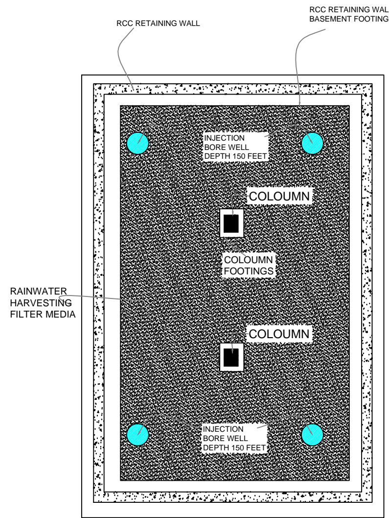
BOTTOM SUMP PLAN
