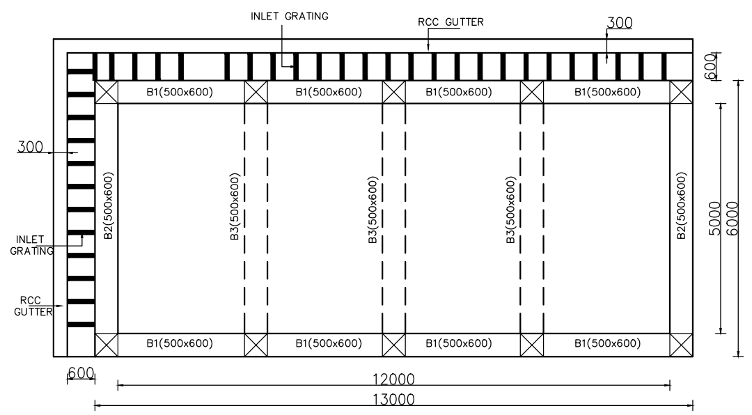
PLAN OF SUMP AT TOP
