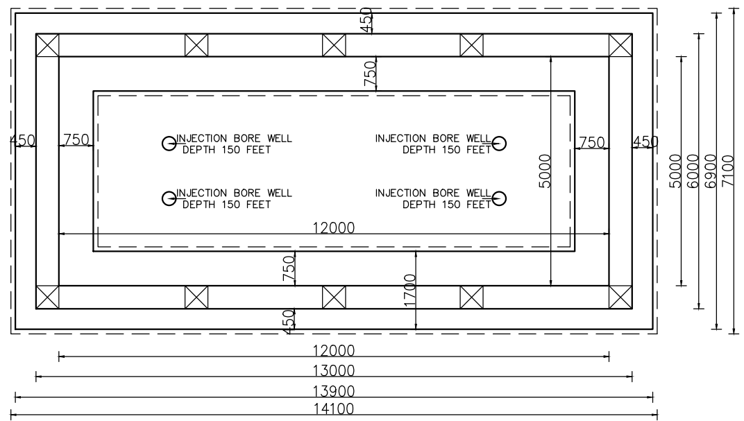
PLAN OF SUMP AT FOUNDATION LEVEL
