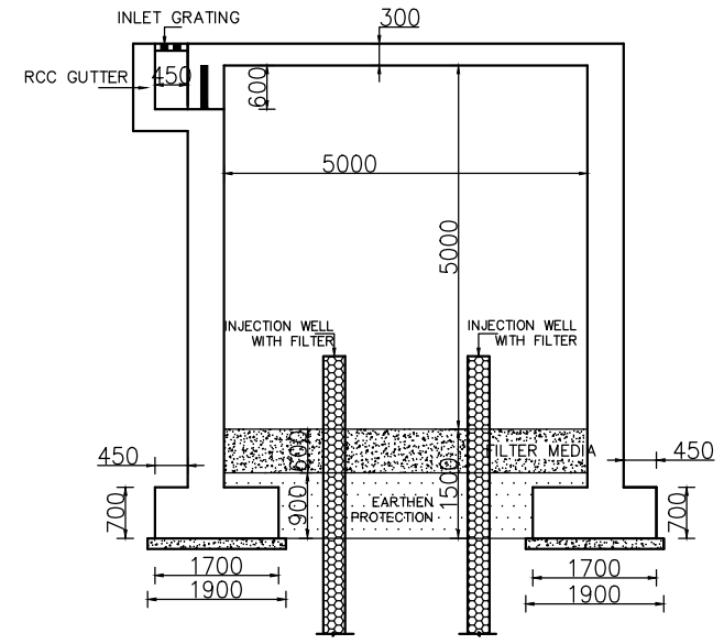
SECTION OF SUMP AT YY
